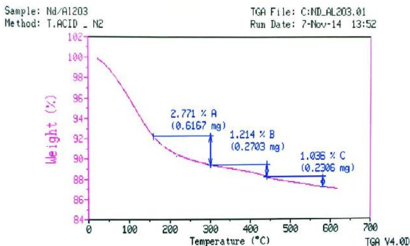
Fig. 4 The loss of DEA with temperature for ZC-Nd catalyst
