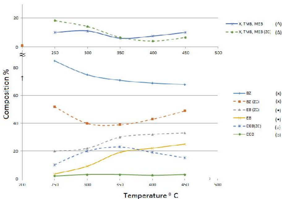
Fig. 7. Concentration of the components in reaction mixture as a function of the temperature catalysts ZC (-----) and ZC-Nd (————). B/E=3/1 mole/mole B(X); EB(•); DEB (o); X+TMB+MEB( )
