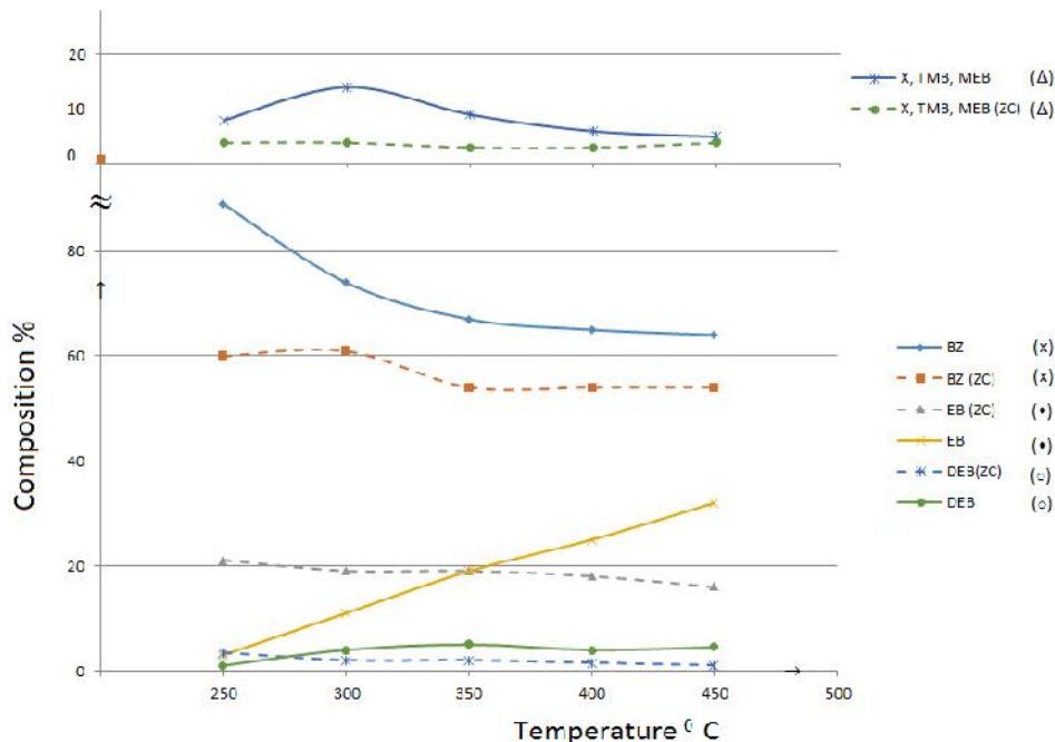
Fig. 6. Concentration of the components in reaction mixture as a function of the temperature catalysts ZC (-----) and ZC-Nd (————). B/E=2/1 mole/mole . B(X); EB(•); DEB (o); X+TMB+MEB( )
