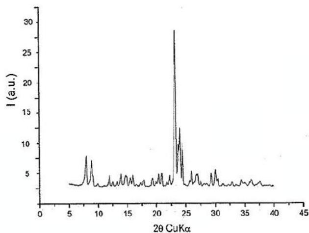
Fig. 2. XRD diffractogram for ZSM-5 zeolite synthesized in the presence of hexamethylenediamine
