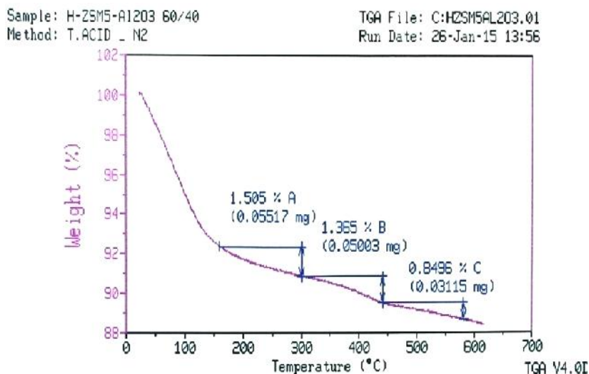
Fig. 3. The loss of DEA with temperature for ZC catalyst
