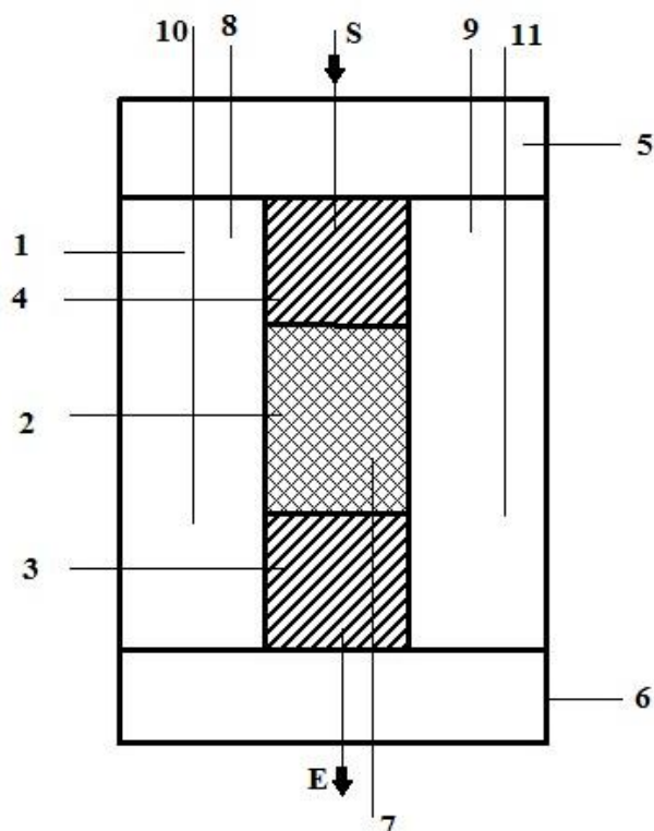
Fig. 1. Alkylation Reactor 1. Reactor Body, 2. Catalyst zone, 3-4 Inert zones, 5-6 Flanges, 7-11 thermocouples, S – reaction mixture supply, E – exit of reaction products
