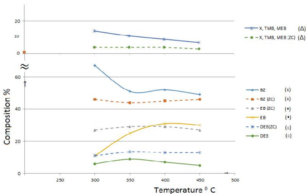
Fig. 5. Concentration of the components in reaction mixture as a function of the temperature catalysts ZC (-----) and ZC-Nd (_____) B/E=1/1 mole/mole B(X); EB(•); DEB (o); X+TMB+MEB( )
