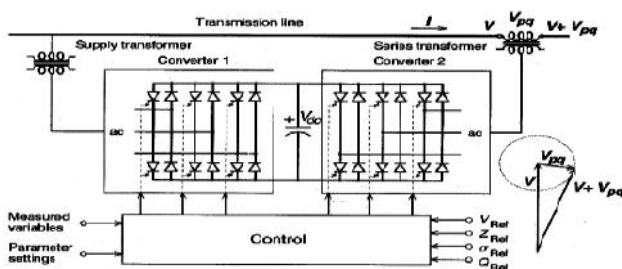
Fig – 3. Unified Power Flow Controller
