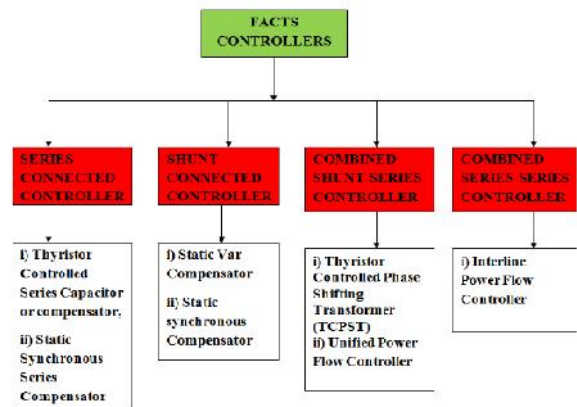
Figure 1: Classification of FACTS Devices
