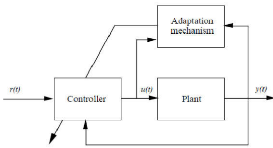
Figure 7. Direct Adaptive control
