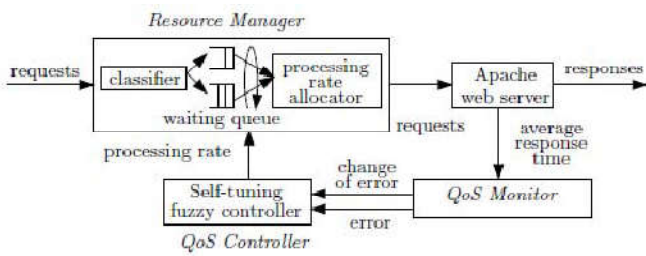
Figure 11. System Architecture of Apache Server STFC
