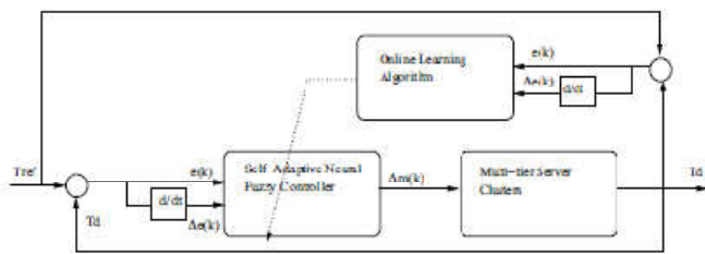
Figure 16. Self adaptive Neuro-Fuzzy Feedback Control system
