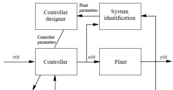
Figure 6. Indirect Adaptive control
