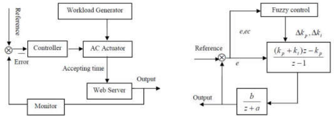
Figure 9. Architecture of ATR Feedback system Figure 10. Fuzzy adaptive control system
