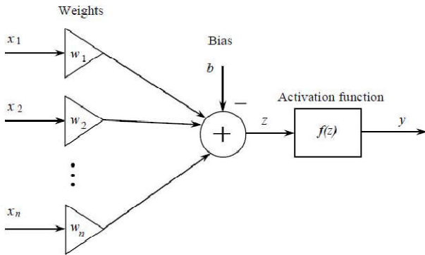
Figure 1. Single Layer Neuron
