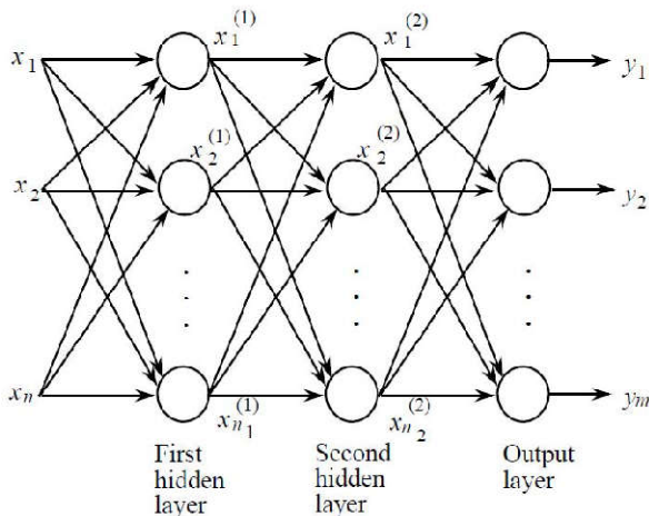
Figure 2. A 3-layer Multi perceptron model
