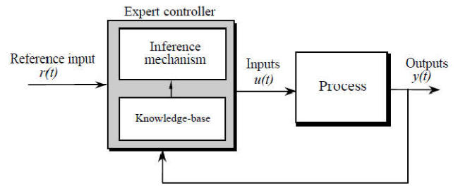
Figure 4. Expert Control System
