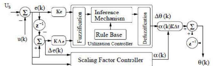
Figure 15. Adaptive Fuzzy PI Controller
