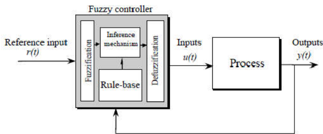
Figure 3. Fuzzy Control System
