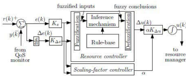
Figure 12. Self tuning Fuzzy Controller
