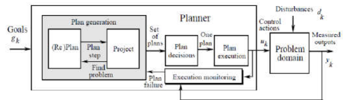
Figure 5. Closed Loop Planning control system
