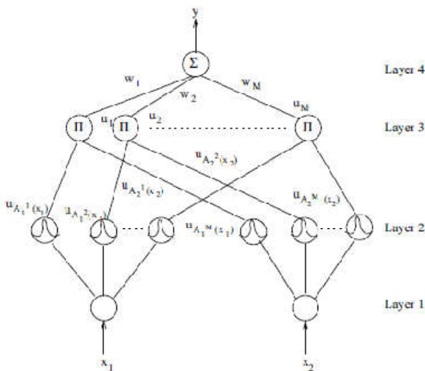
Figure 17. Neuro-Fuzzy Control Schematic diagram
